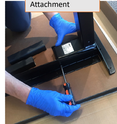
Leg Cross Bracket Alignment and Attachment
